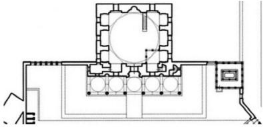
İstanbul Hadim İbrahim Paşa Camii (1551) Mimar Sinan
